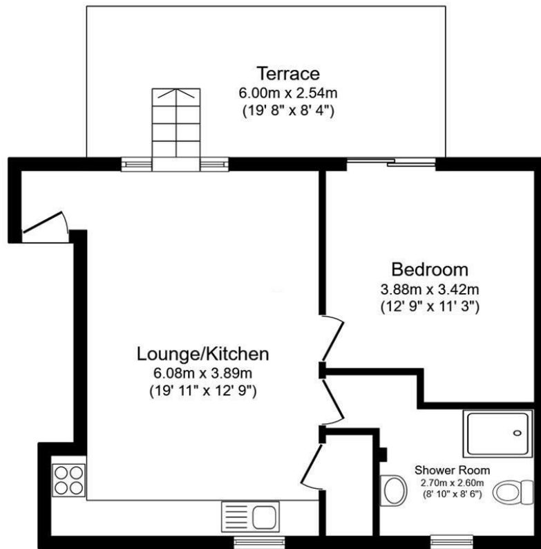
Floor Plan
